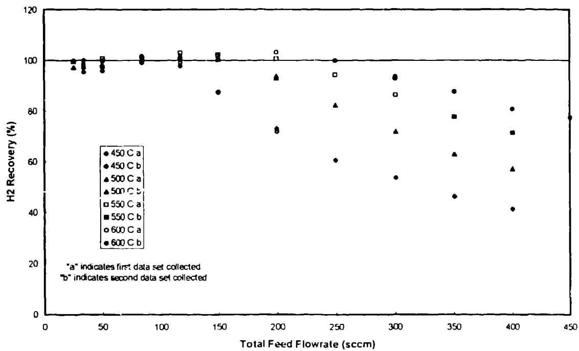
Figure 3 Water-Gas Shift Hydrogen Recoveries Using a Feed Composition of \text{CO}:\text{H}_2\text{O} = 1.5:1 , at various Flowrates and Temperatures
