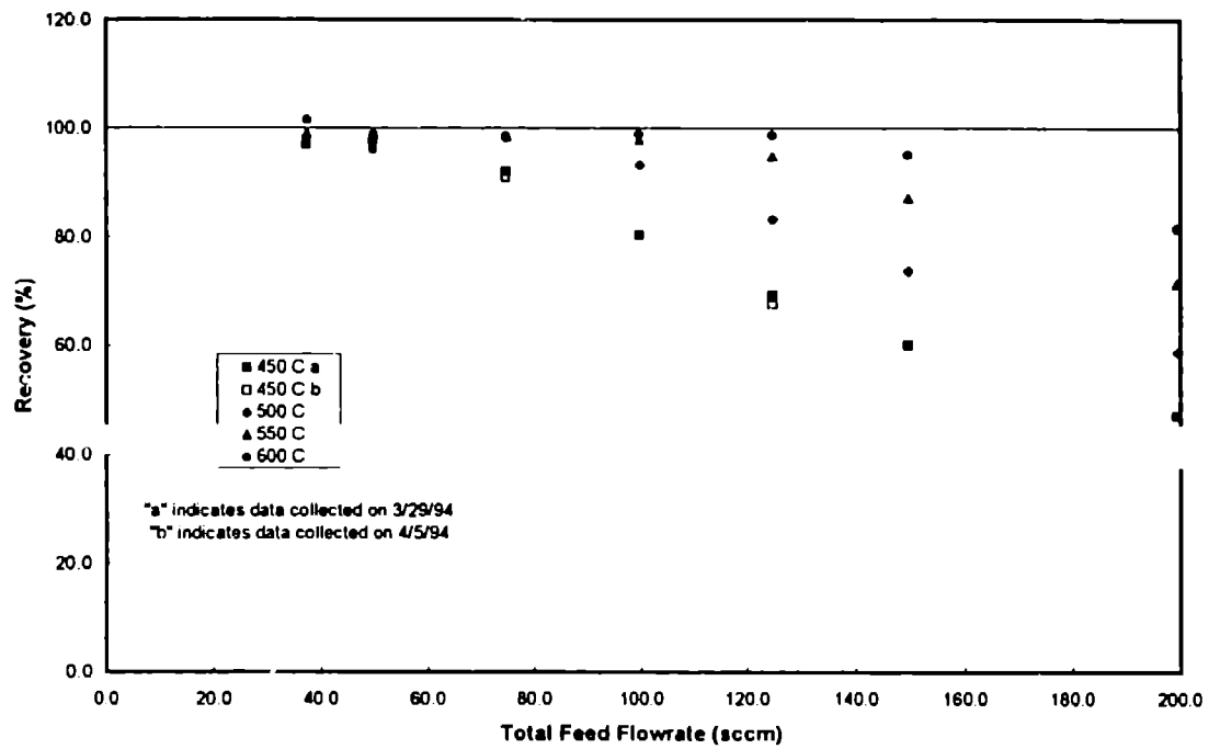
Figure 7 Steam Reforming Hydrogen Recoveries Using a Feed Composition of CH 4 :H 2 O = 1:1.5, at various Flowrates and Temperatures
