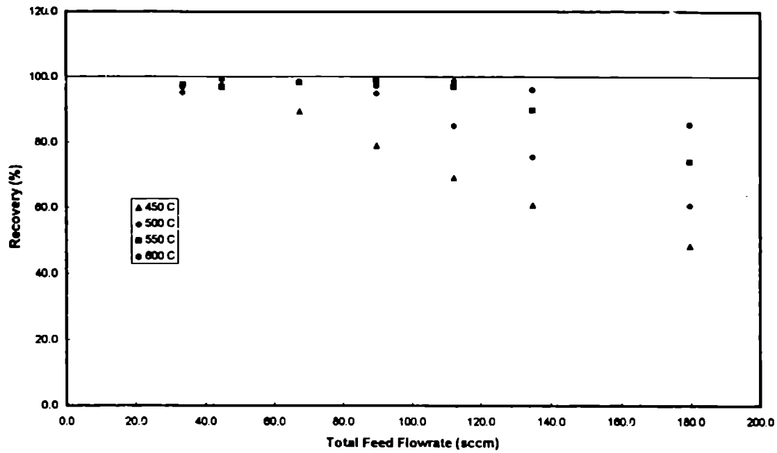
Figure 6 Steam Reforming Hydrogen Recoveries Using a Feed Composition of CH 4 :H 2 O = 1:1.25, at various Flowrates and Temperatures
